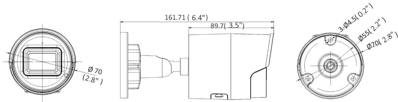
Unit: mm(Inch)
